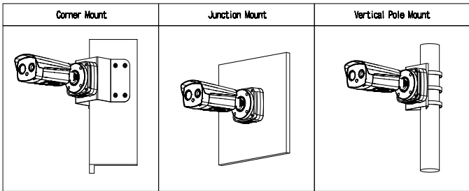
PFA154 Vertical Pole Mount Bracket
