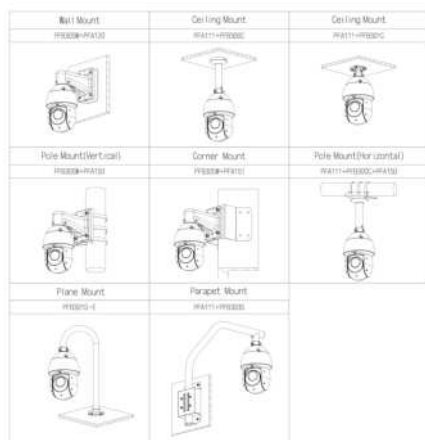
DH-PFB303S Parapet Mount Bracket
